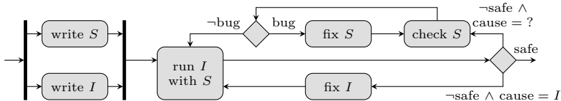
Fig. 4: Intended workflow of discourje
