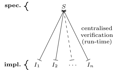
Fig. 2: Discourje (this paper)
