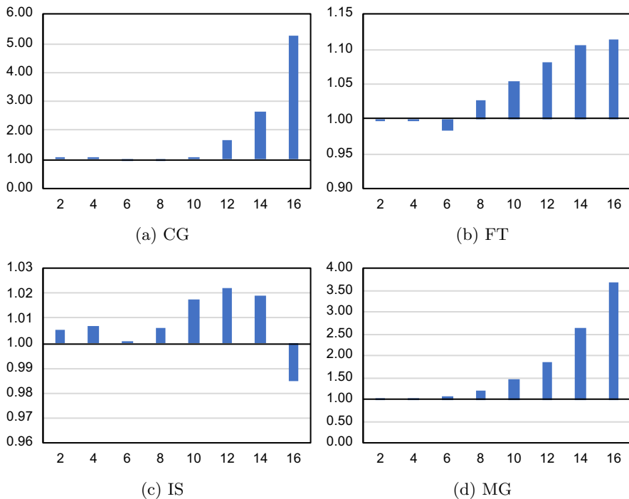
Fig. 23: NPB: slowdown of running implementations with monitoring enabled relative to running them without monitoring enabled (y-axis) as the number of worker threads increases (x-axis), as a measure of overhead
